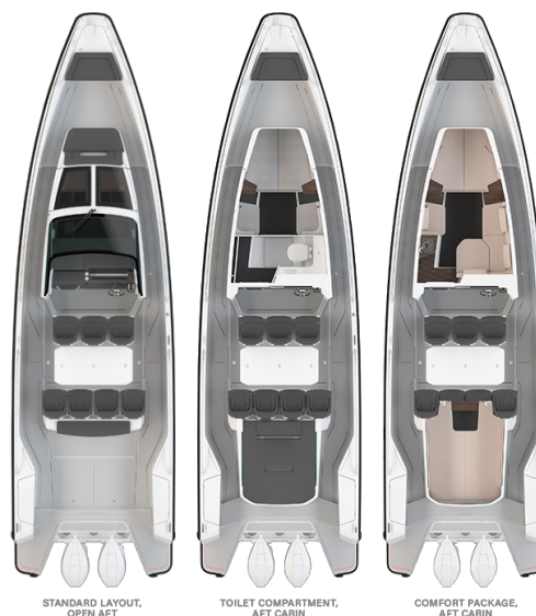
STANDARD LAYOUT, OPEN AFT
